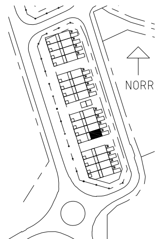
SITUATIONSPLAN
