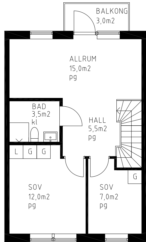
PLAN 1 TR
